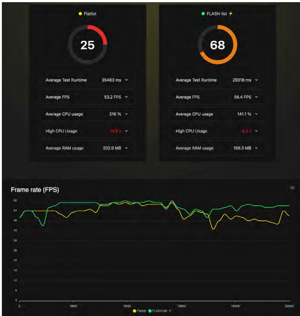
Performance report from Bamlab's Flashlight
