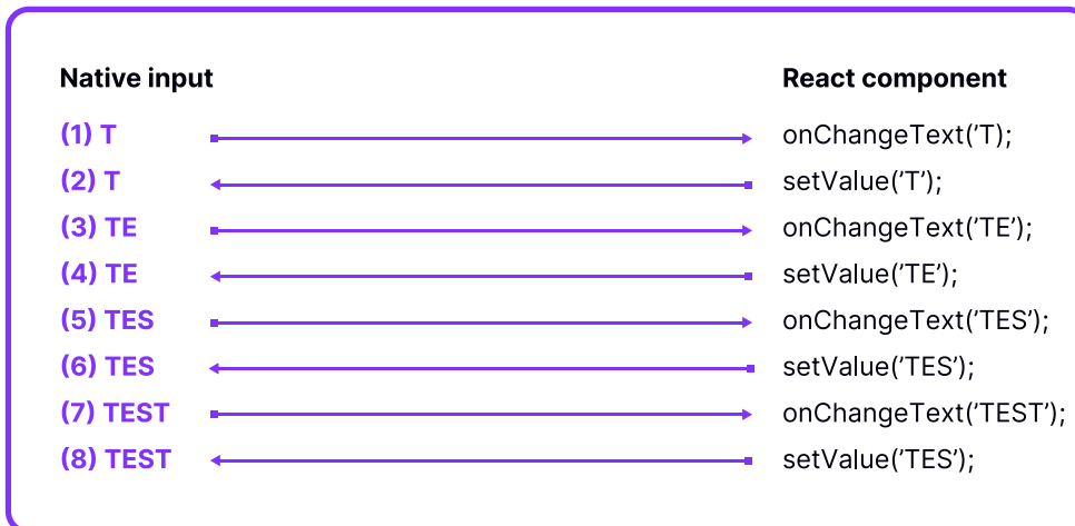
Diagram that shows what happens while typing TEST
