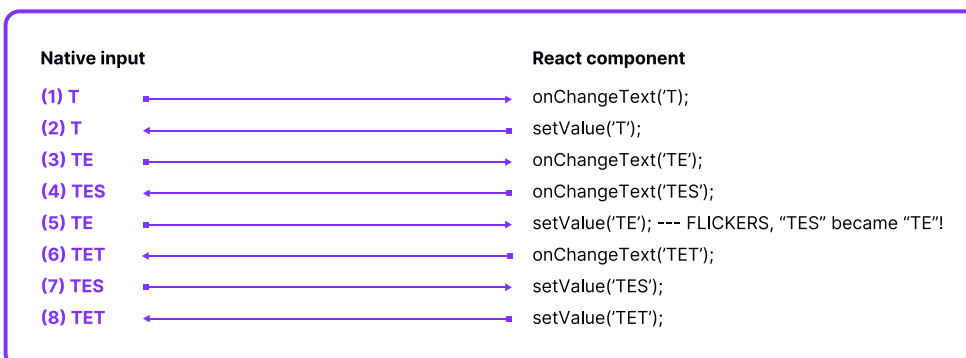
Diagram that shows what happens while typing TEST too fast
