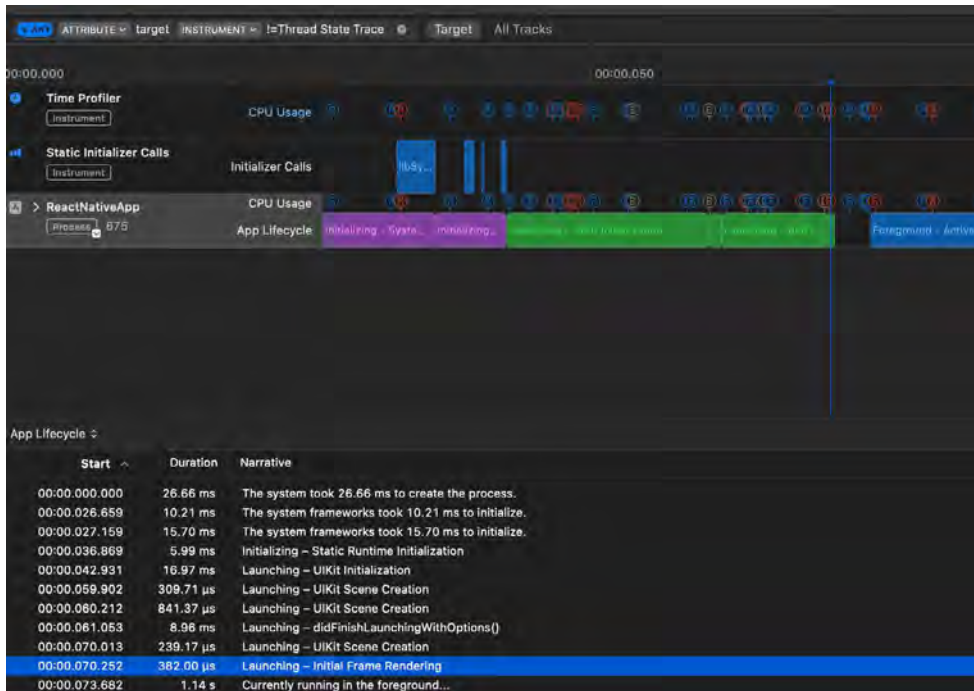
Example usage of Xcode's App Launch tool
